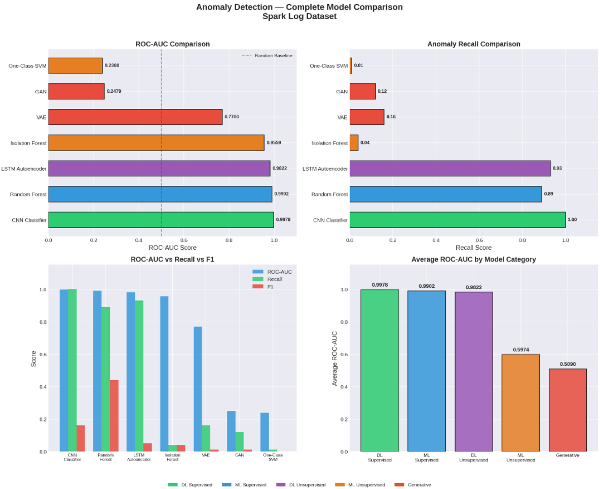
Figure 22 Spark logs Model Comparison
