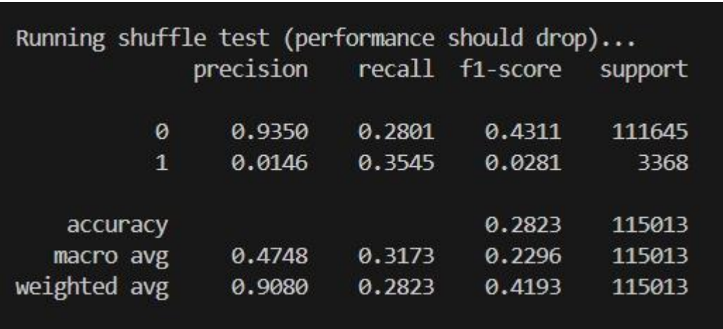
Figure 3 Shuffling Test Performance
