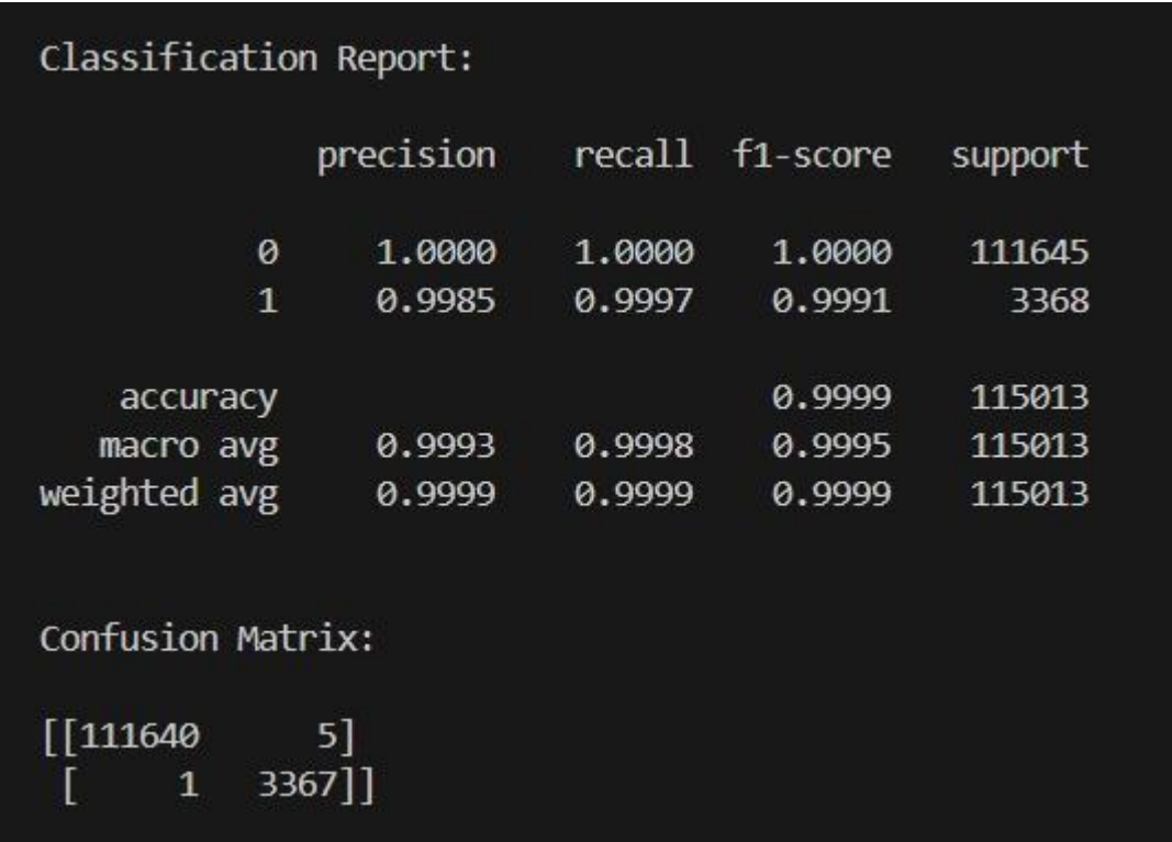
Figure 2 HDFS ML XGBoost Confusion Matrix
